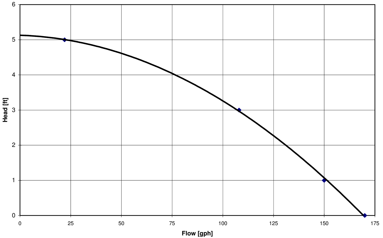
P140 Pump Curve Magnetic Driven Pump
