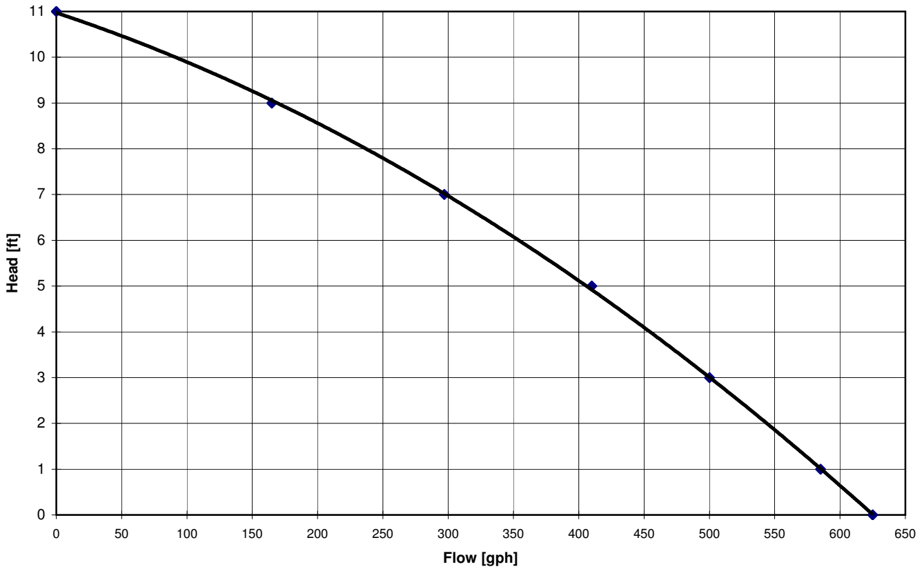
P600 Pump Curve Magnetic Driven Pump
