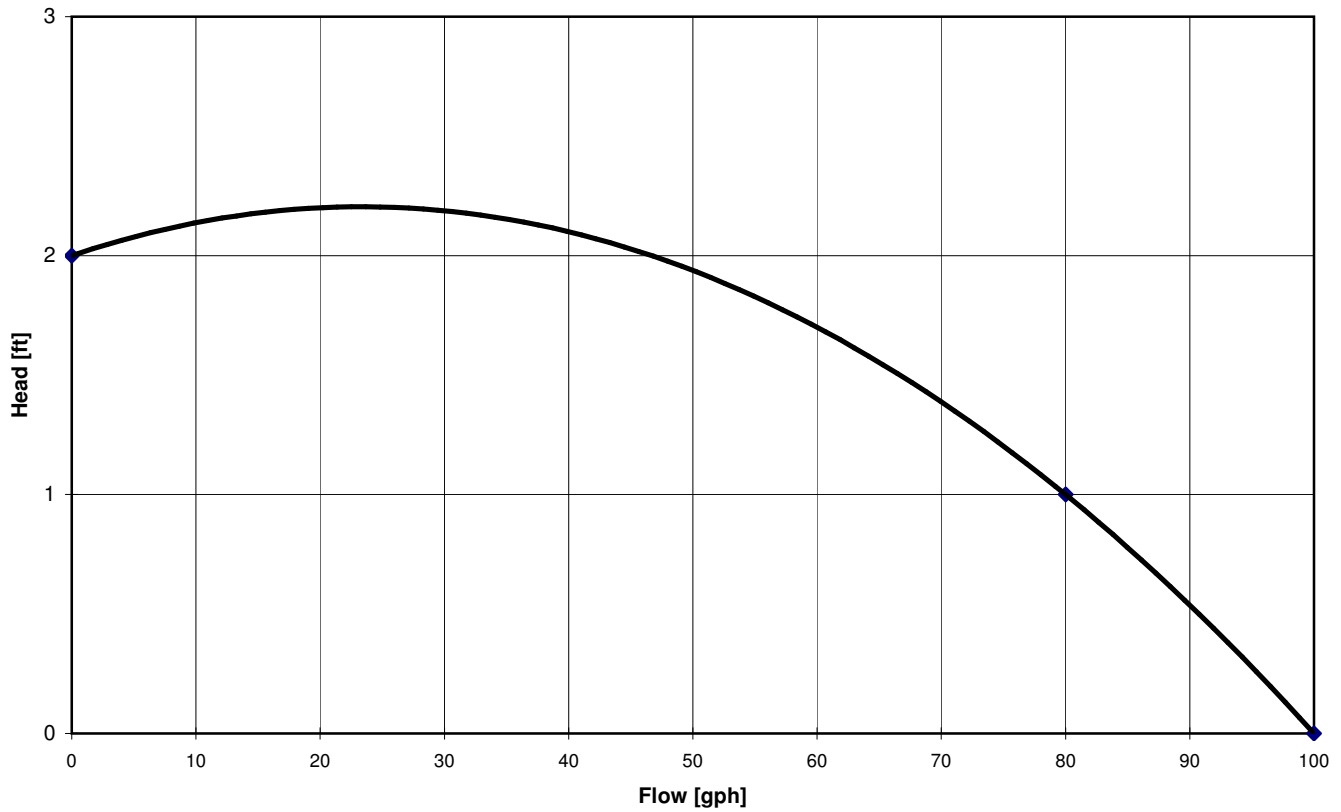
P80 Pump Curve Magnetic Driven Pump
