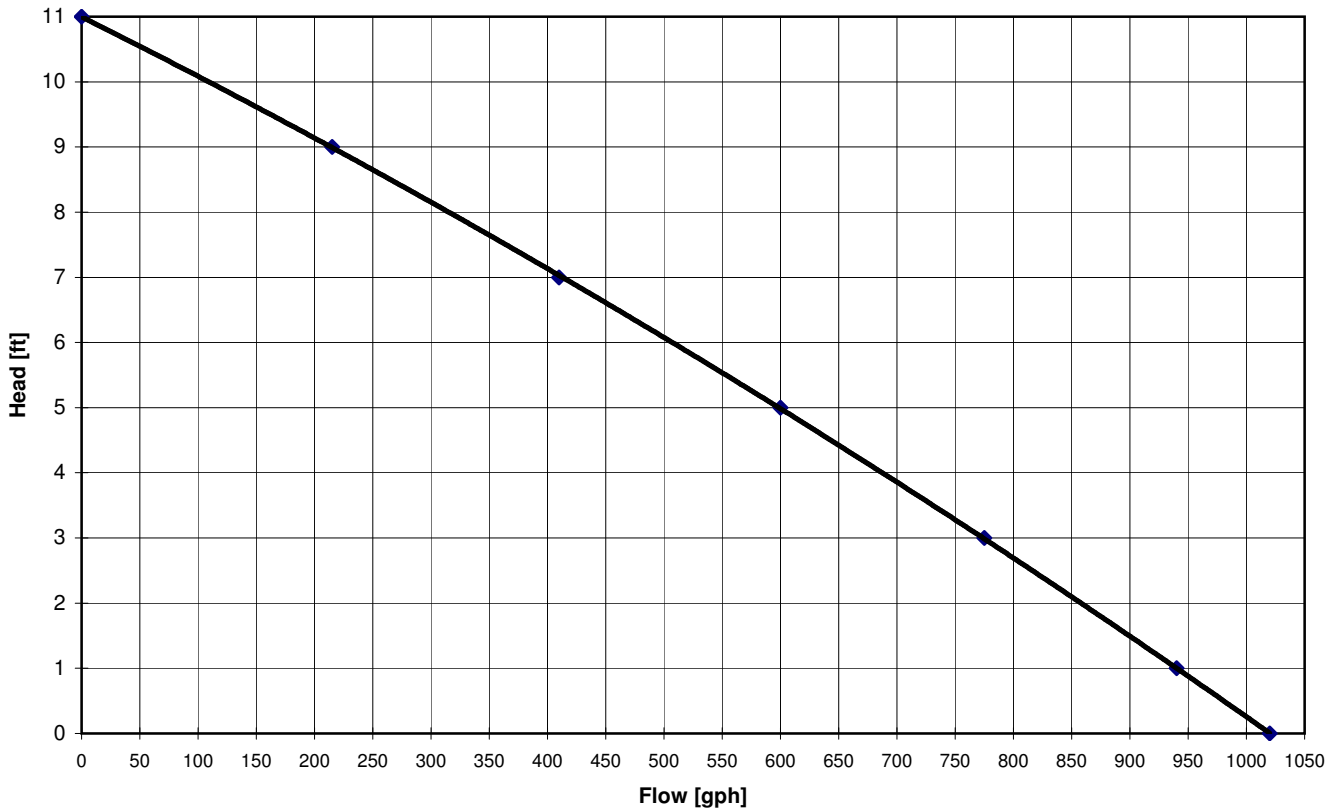
P900 Pump Curve Magnetic Driven Pump
